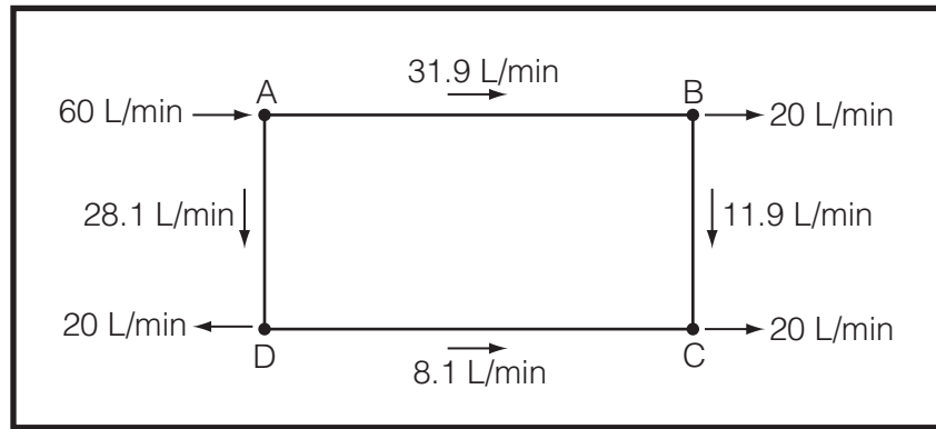
Figure 2.3: Flow distribution
