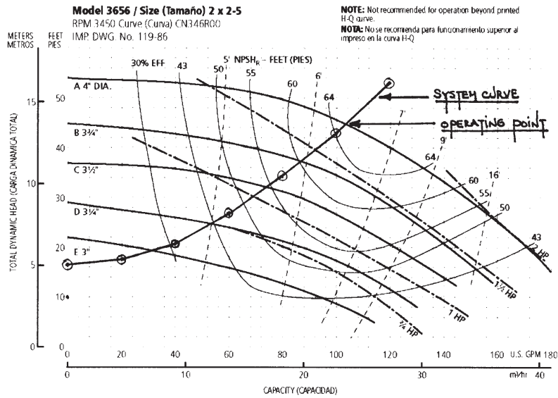
Figure 2.9: System Curve on Pump Curve.
