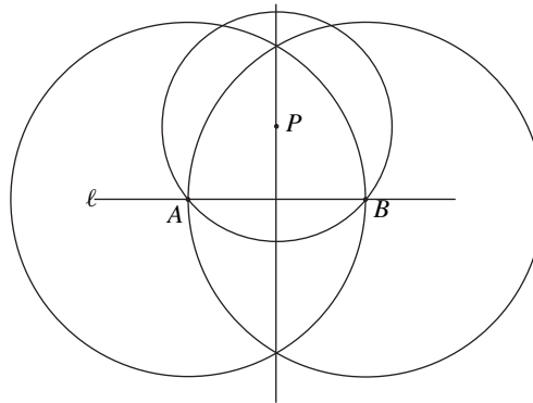
FIGURE S1.4: Exercise 1.6(b) Construction of a line through P , perpendicular to \ell
