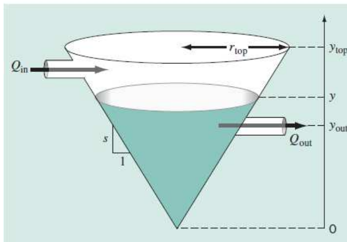
FIGURE P1.11
