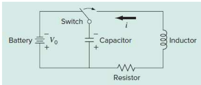
FIGURE P2.11
