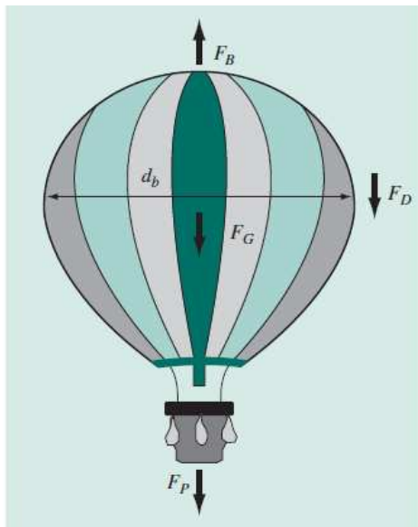
FIGURE P1.28
