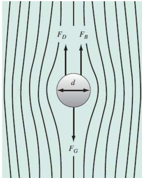
FIGURE P1.22
