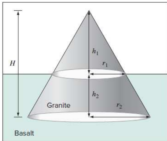
FIGURE P1.25
