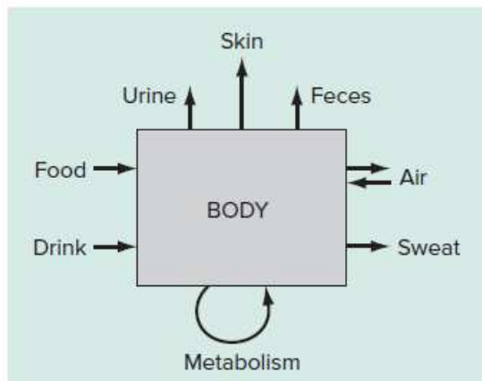
FIGURE P1.13
