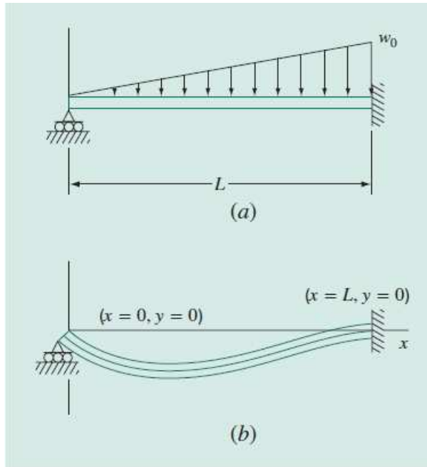
FIGURE P2.26
